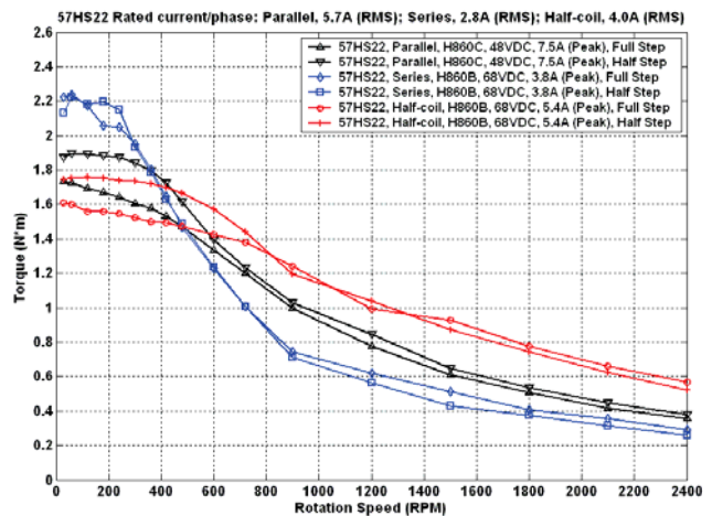
Figure 9: Speed-torque curves of the 57HS22
