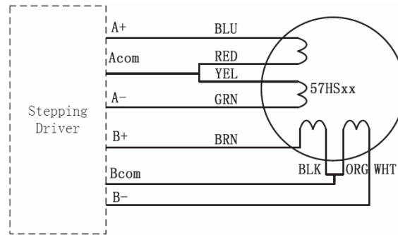
(e) 57HSxx unipolar connection (8 leads)
