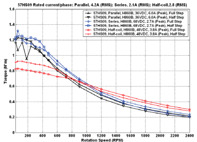
Figure 7: Speed-torque curves of the 57HS09
