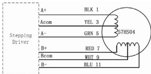
(a) 57HS04 unipolar connection
