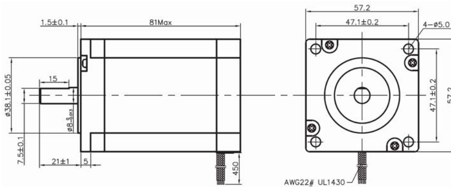
Figure 4: Mechanical specification of 57HS22
