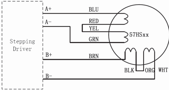
(c) 57HSxx series connection (8 leads)
