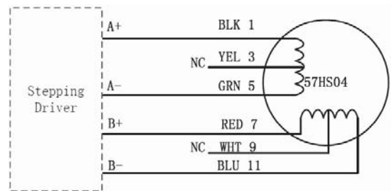
(b) 57HS04 bipolar (series) connection
